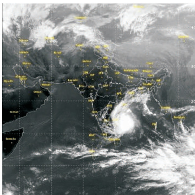
Monitoring of Cyclon "Vardah" by INSAT-3DR image
